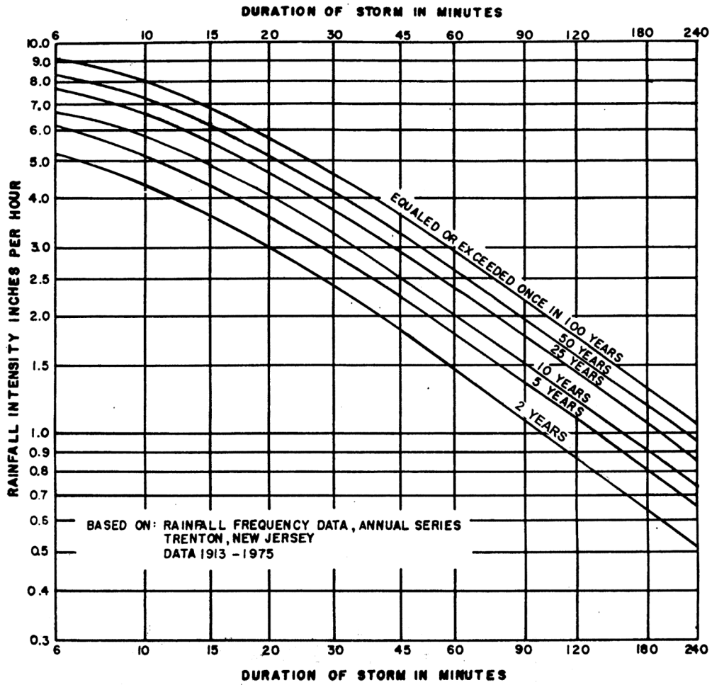
Figure 5-4: Rainfall Intensity-Duration-Frequency Curve
