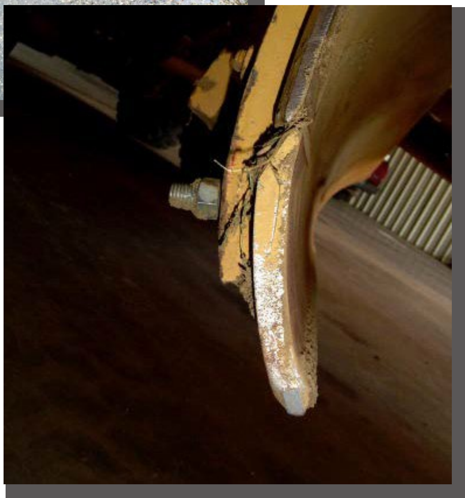
Example of carbide-insert in a cutting edge with hard facing on the bottom of the face to increase wear life.
