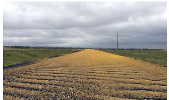
Typical washboard damage on an unpaved road (Source: Jo Michele Sheridan).
