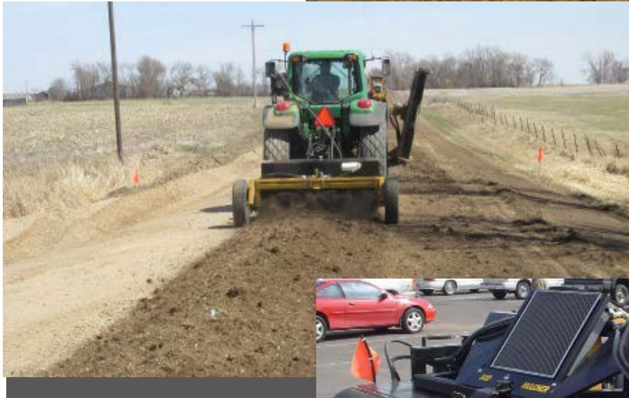
Reshaping, or reconstructing a gravel road requires processing of very large windrows of material. Examples of two commercially marketed pulverizers on the market which speed the gravel reclaiming process.
