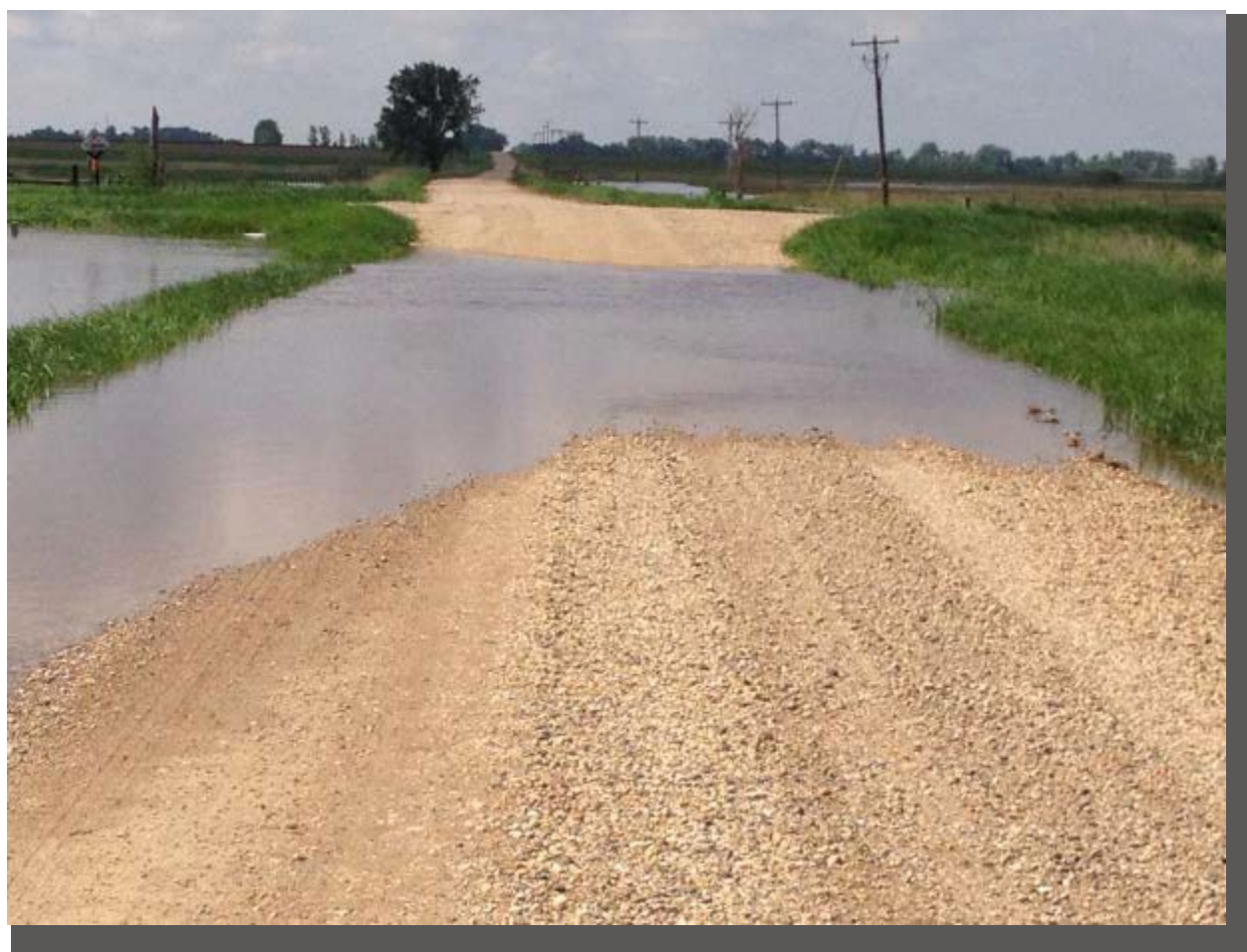
Plugged or collapsed culverts cause serious damage when water flows over roads.
