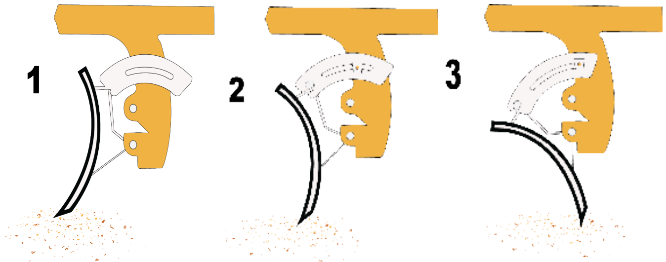
FIGURE 2: Moldboard pitch.
