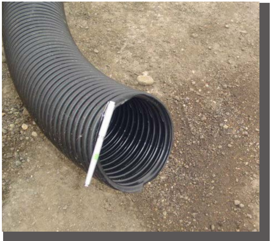
Common flexible polyethylene drainage pipe is plowed below the surface and brought out to the surface on the foreslope at regular intervals to complete this work.
