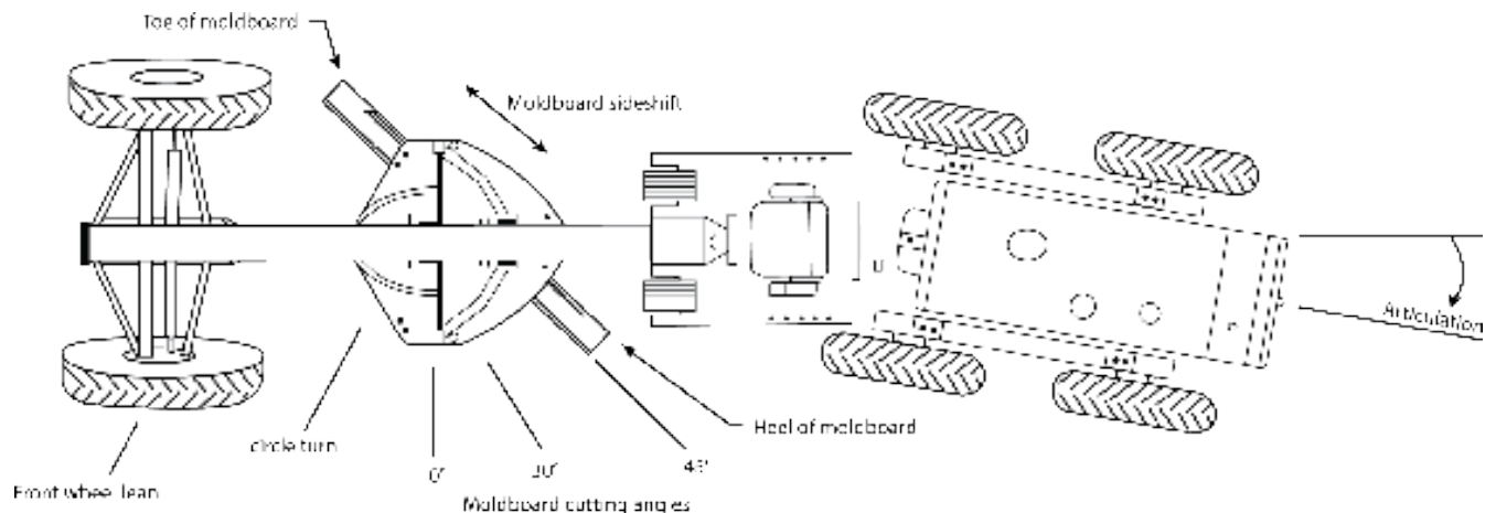
FIGURE 3: Articulated Motorgrader
