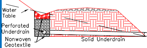
FRENCH DRAIN
