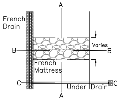
FRENCH DRAIN
